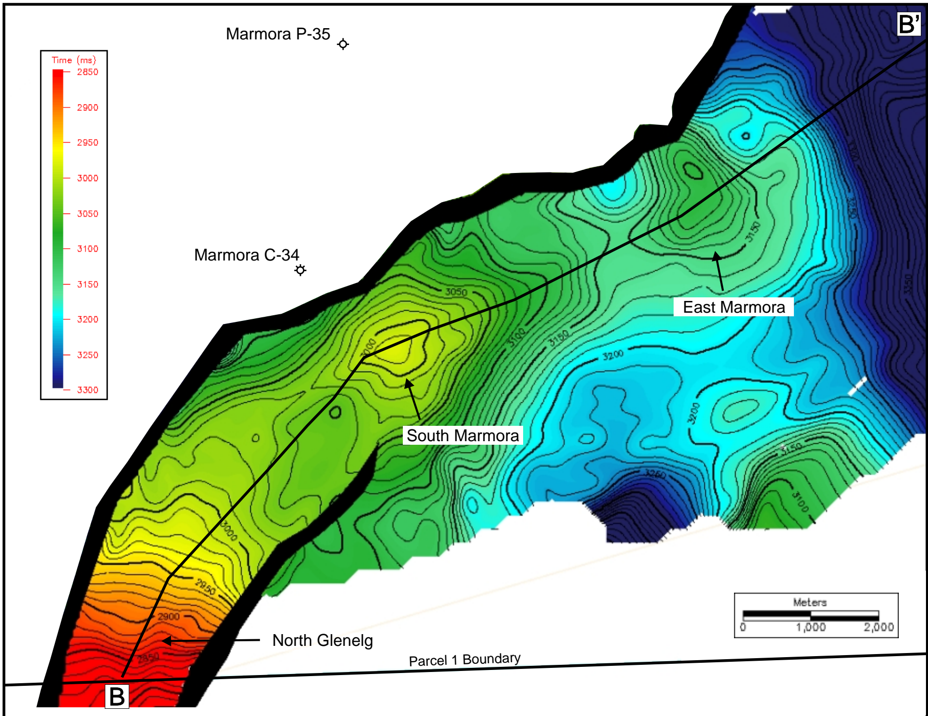
Structure map of a lower Mississauga seismic marker and the location of seismic profile B-B' through the North Glenelg, South Marmora and East Marmora prospects.
